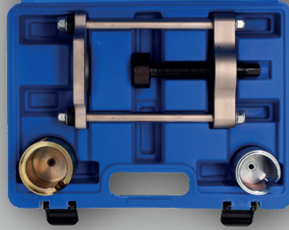
BT671900 Front axle transverse link bush tool for VAG
